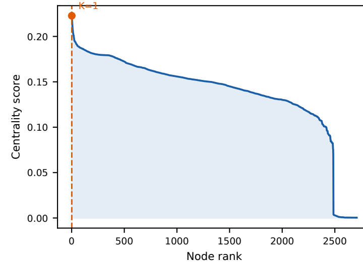
Citeseer x Closeness
