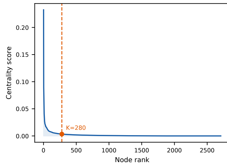
Citeseer x Betweenness
