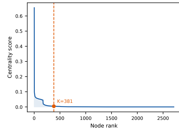
Citeseer x Eigenvector
