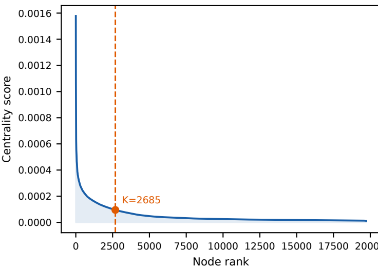
Pubmed x PageRank
