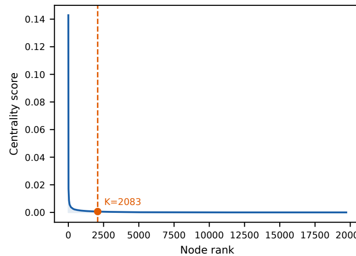
Pubmed x Betweenness
