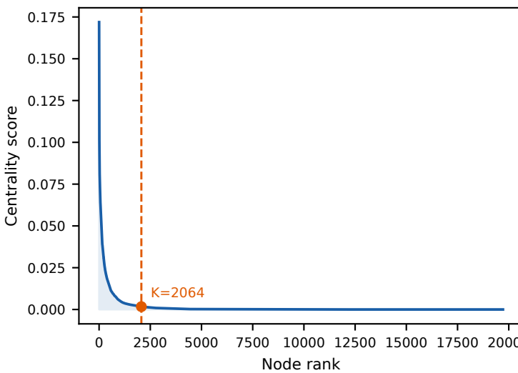
Pubmed x Eigenvector
