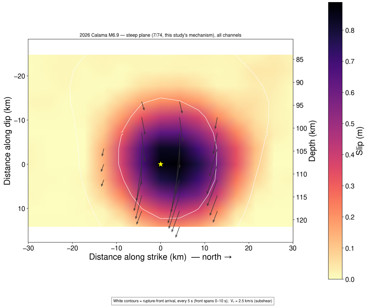
Figure 10: The conjugate model (steep plane 7/74): nearly equal misfit, same moment and mechanism, mirrored geometry. Given that the well-constrained large events of this cluster (2024 M7.4; possibly 1950 M8.2) ruptured steep planes, the steep-plane model is shown below with the same completeness as the preferred model.
