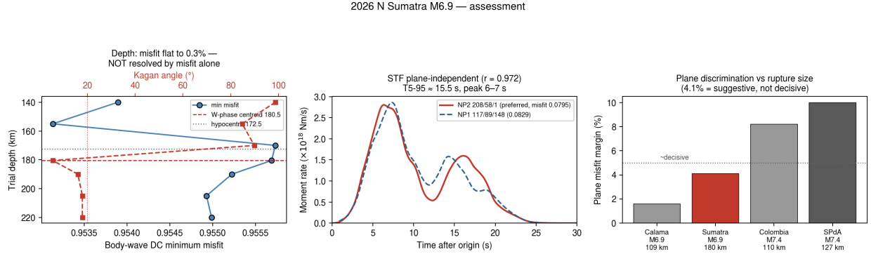
Figure 8: Left: the depth scan — misfit (blue) is flat to 0.3 % across 140–220 km, but the Kagan angle (red) reveals a sharp transition: the mechanism is chaotic at 140–170 km ( 85\text{--}99^\circ ) and locks onto the W-phase from 180.5 km downward ( 5.5\text{--}18^\circ ). Centre: the source-time function is plane-independent. Right: the plane-discrimination margin in the project’s rupture-size context.
