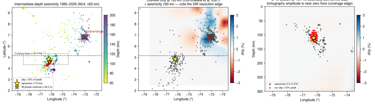
Figure 12: Left: intermediate-depth seismicity; the rupture (red) lies inside the NNE-trending Cauca cluster, which terminates at the Caldas tear ( \sim 5.15^\circ\text{N} ); the Bucaramanga nest is the dense knot 407 km NE. Centre: CARMA dV_p at 120 km — the strong fast anomaly underlies Bucaramanga (the Caribbean slab of Sun et al. 2022); amplitude at our event is \sim 0.01\% (SW resolution edge). Right: E–W section at 4.84^\circ\text{N} — the slip patch (85–125 km) sits exactly on the east-dipping seismicity band that defines the local Nazca slab.
