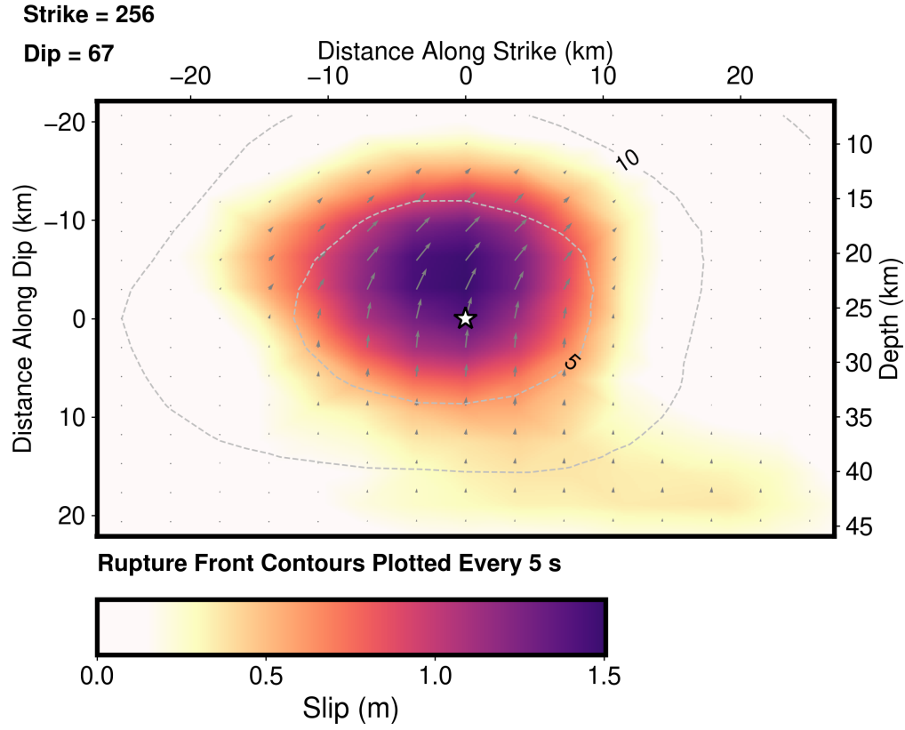
Figure 6: Preferred (steep-plane) slip model. Star: hypocentre; contours: rupture front every 5 s; arrows: slip direction (reverse). Peak 1.46 m, slip at 17–37 km depth.
