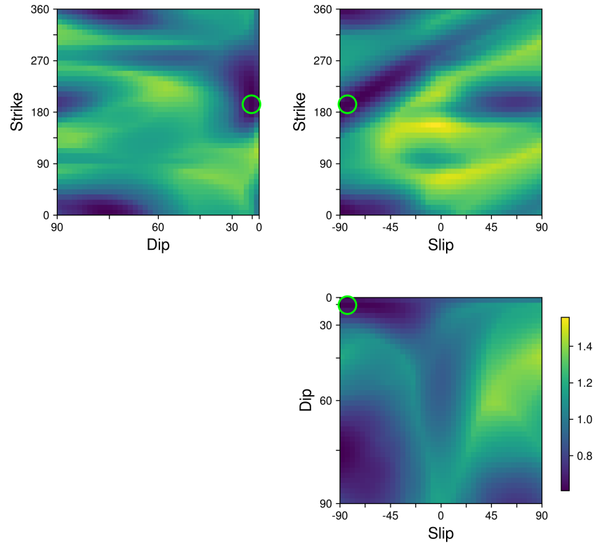
Figure 6: DC misfit surfaces (strike–dip–rake) for the final joint search.
