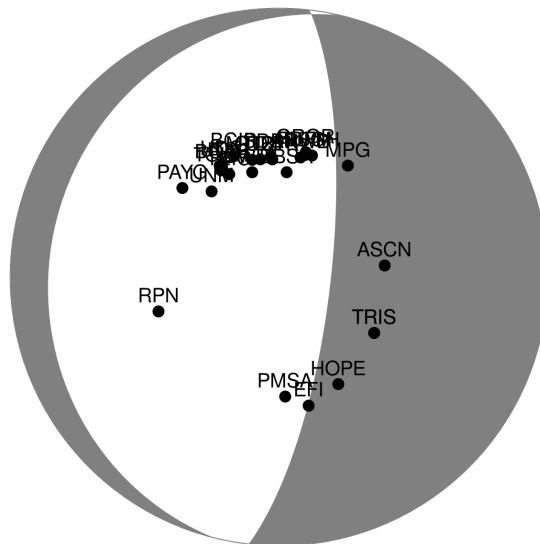
Figure 5: Final DC (194/16/−83; body 25–60 s + surface waves, 107 km) and the 26 stations.
