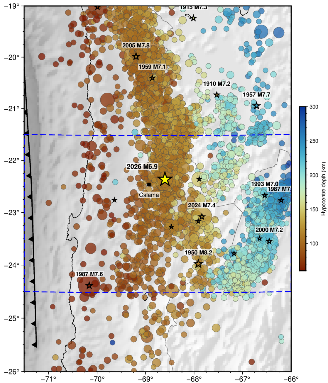
Intermediate-depth seismicity (USGS, M \geq 4.5 , z \geq 60 km)
