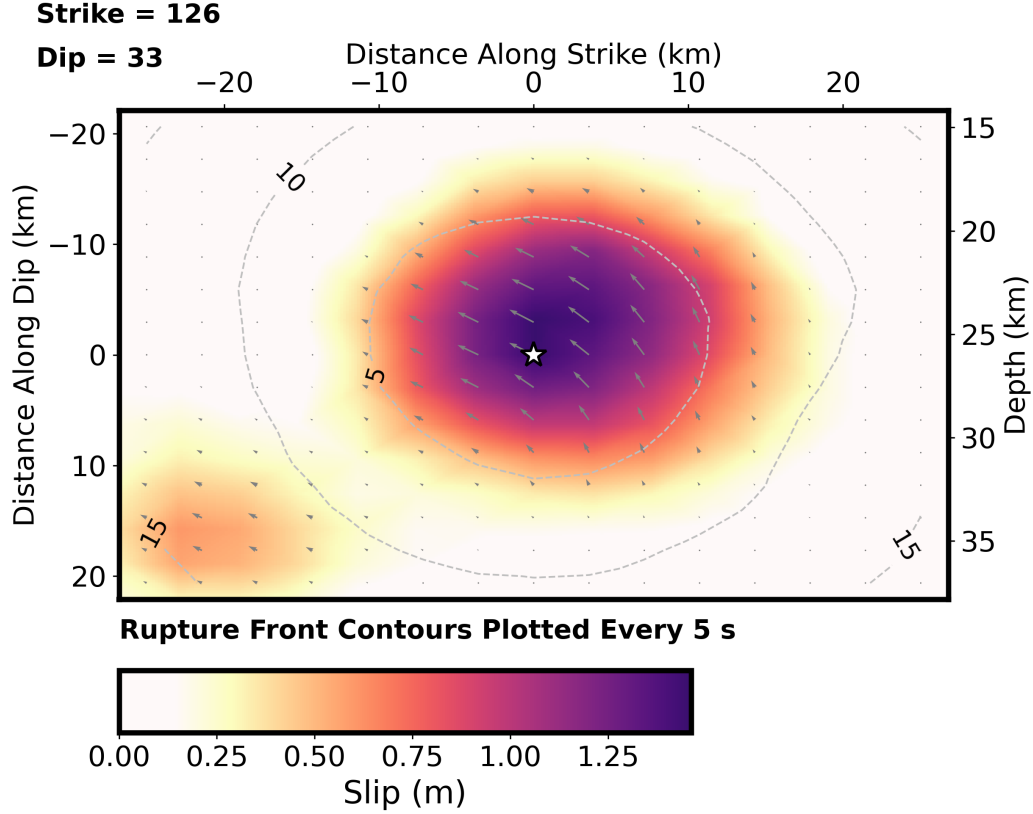
Figure 6: Preferred (steep-plane) slip model. Star: hypocentre; contours: rupture front every 5 s; arrows: slip direction (reverse). Peak 1.46 m, slip at 17–37 km depth.
