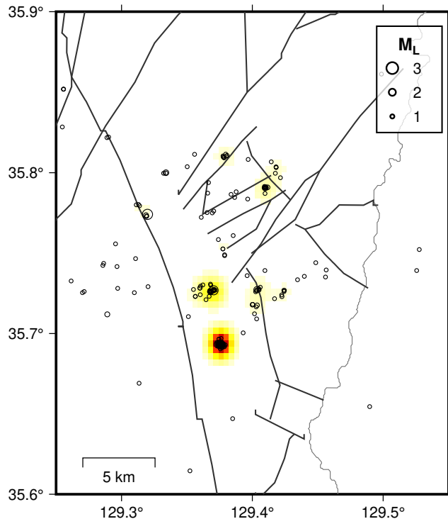
6 months after 2016 Gyeongju (224 events, 13 stations)
