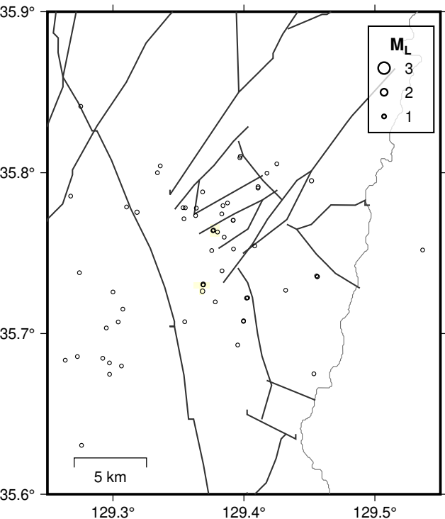
6 months before 2016 Gyeongju (66 events, 13 stations)
