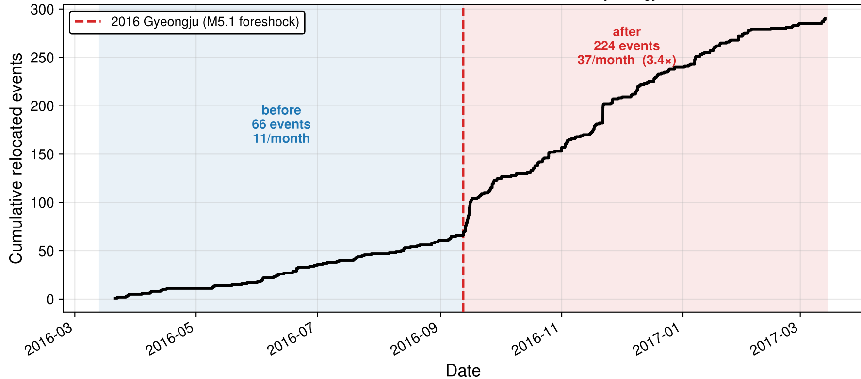
Ulsan Fault — cumulative count across the 2016 Gyeongju window
