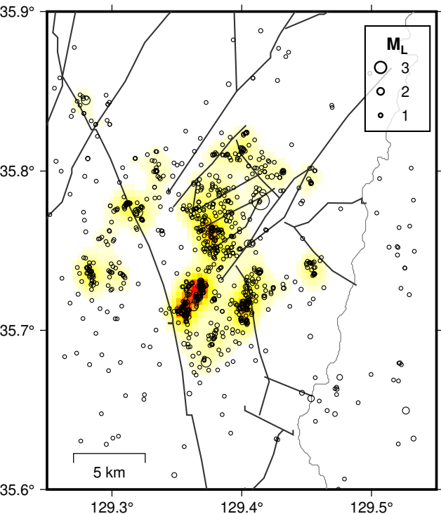
Background seismicity (1017 events)
