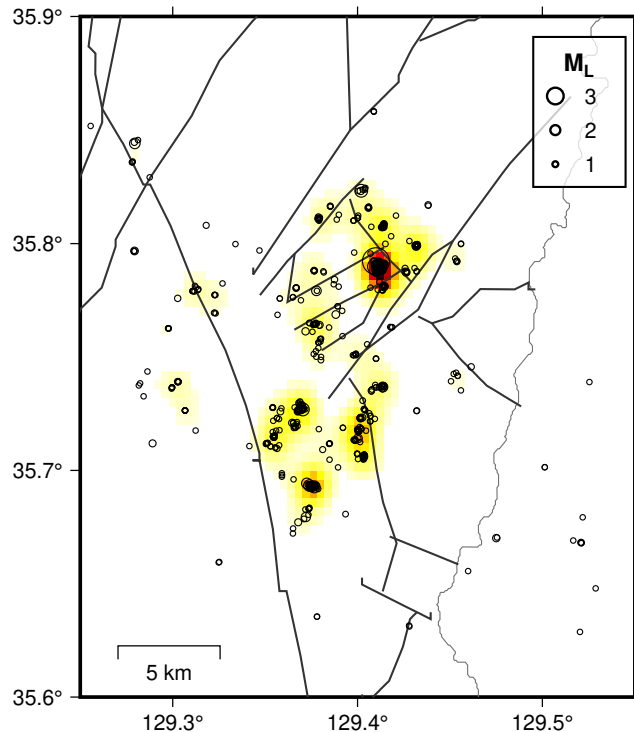
Clustered seismicity (667 events)
