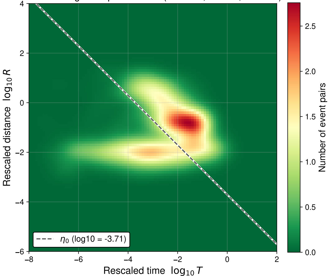
Nearest-neighbour pairs in R–T (3D NND, b = 1.0 , D_f = 1.1 )
