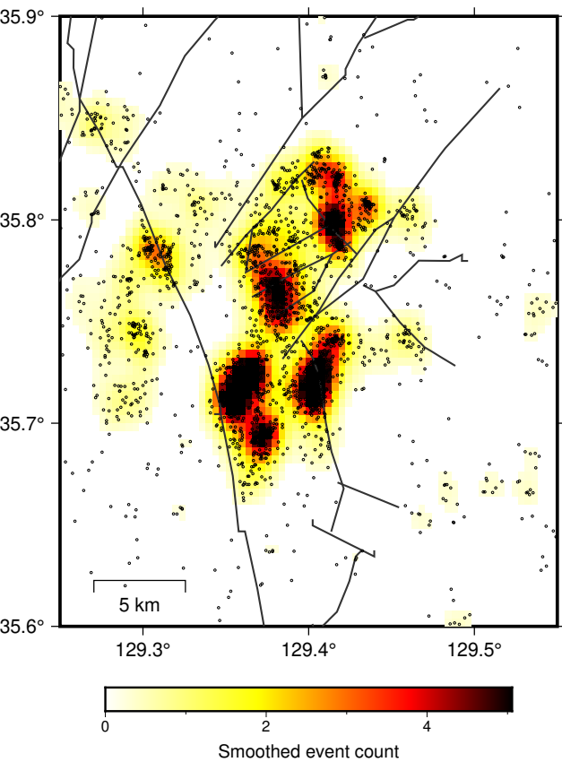
Seismicity count density
