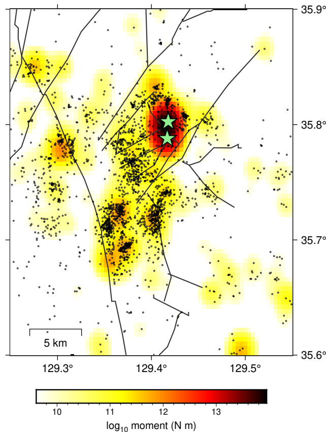
Seismic moment release
