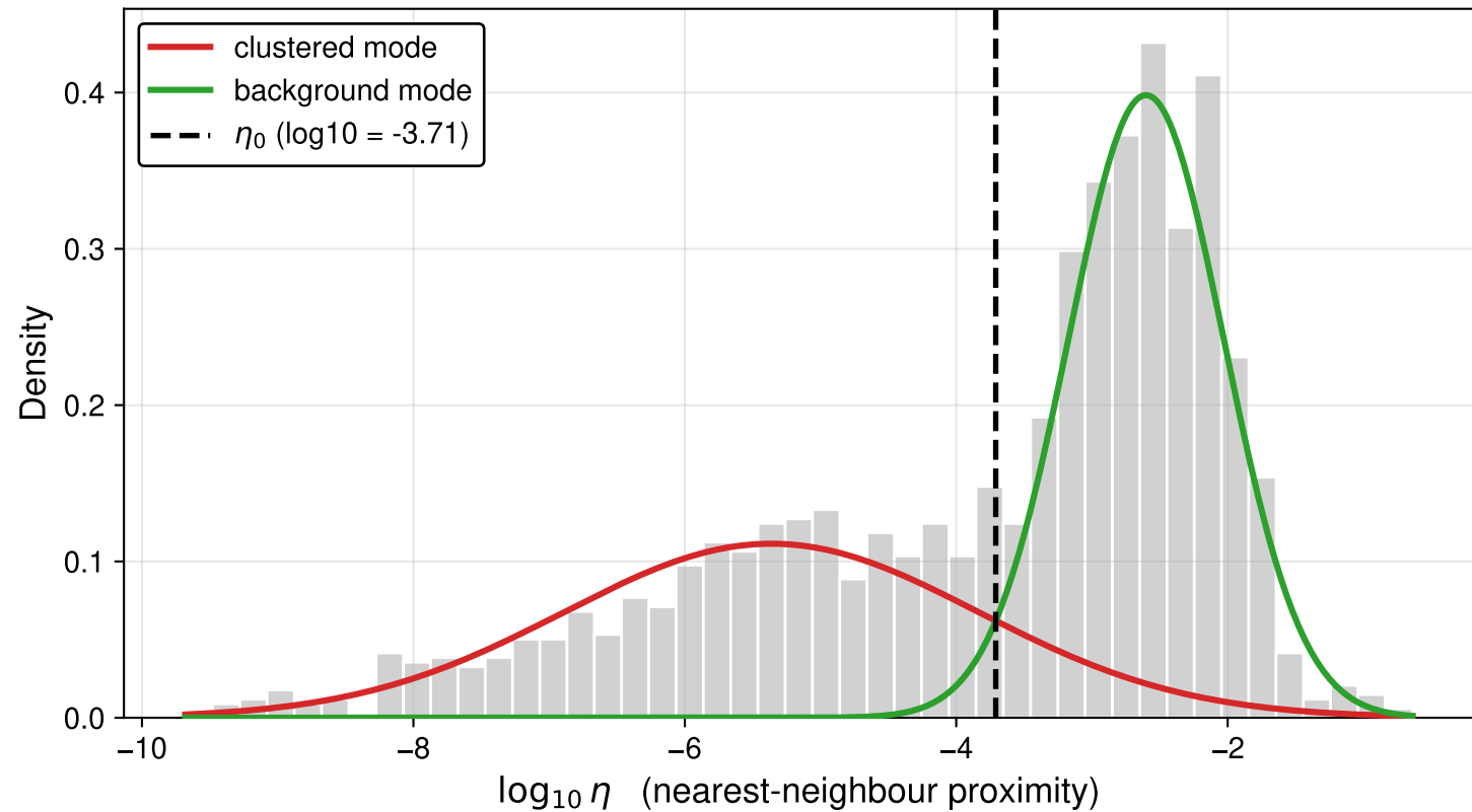
1-D bimodal NND distribution + GMM (3D, Df = 1.2, b = 1.0)
