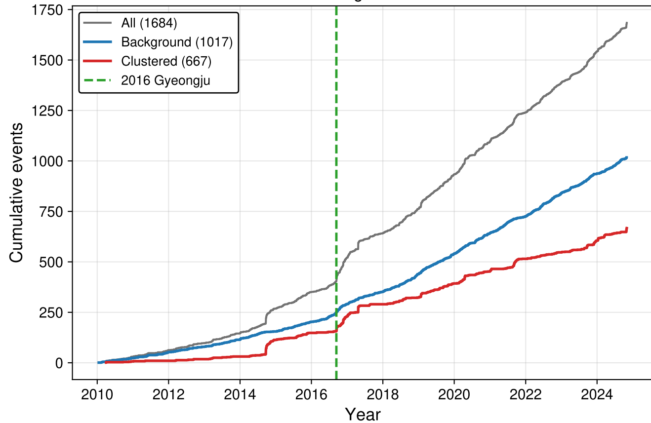
Cumulative: background vs clustered
