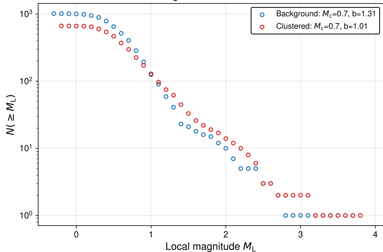
Magnitude distributions
