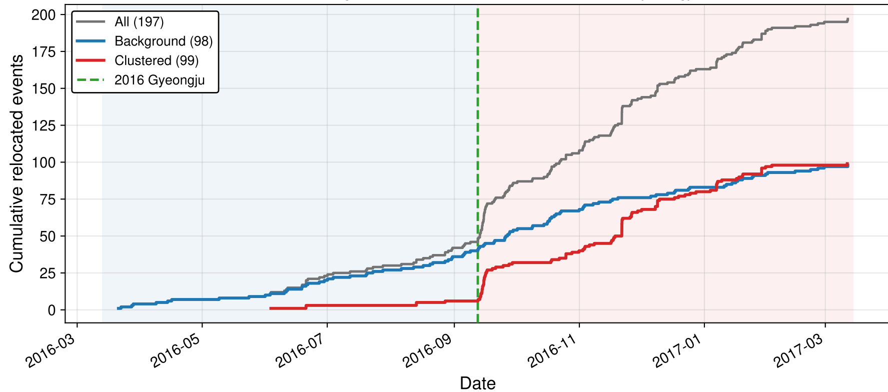
Ulsan Fault — background vs clustered across the 2016 Gyeongju window
