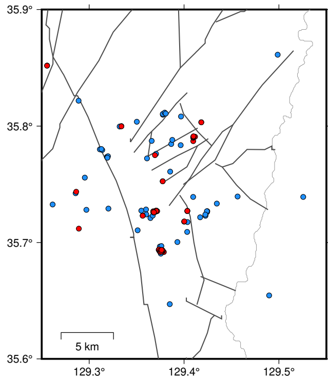
6 months after Gyeongju (background 58, clustered 93)
