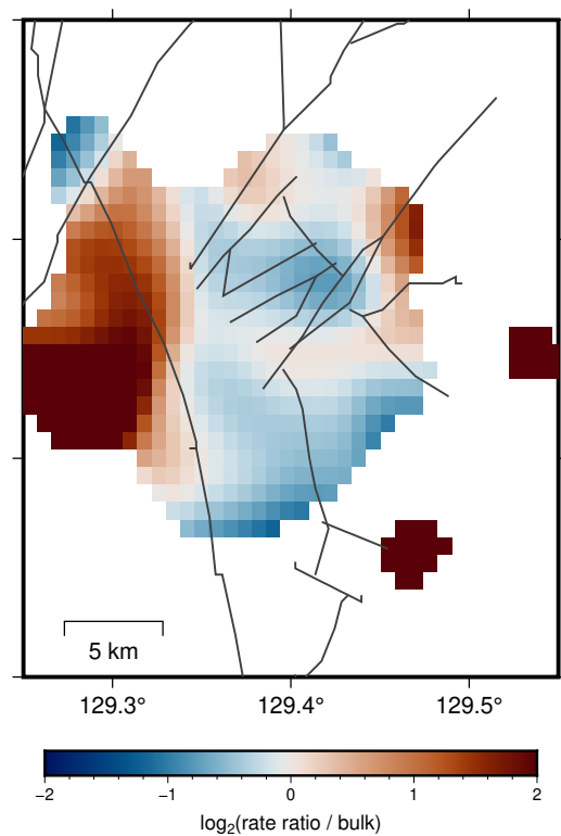
Change relative to mean (log 2 )
