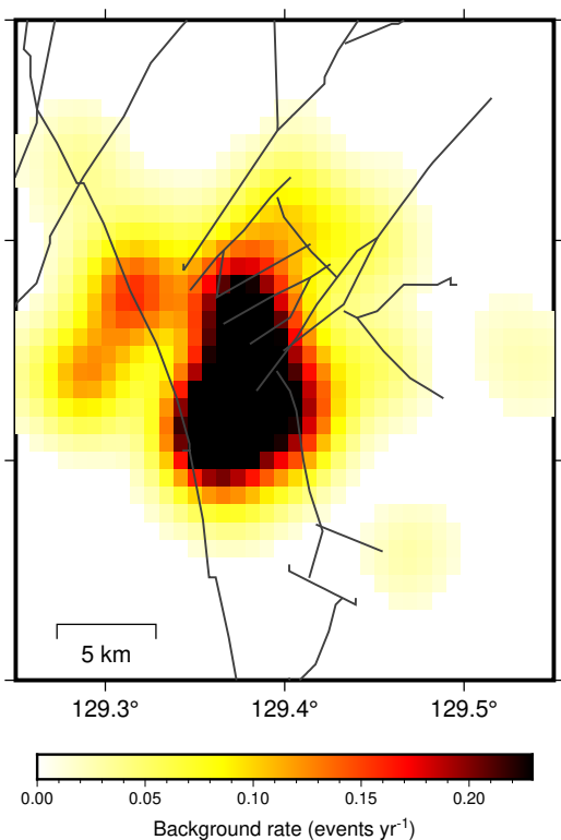
Background rate after (N=463)
