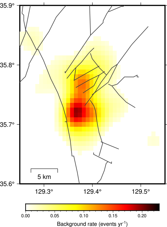
Background rate before (N=151)
