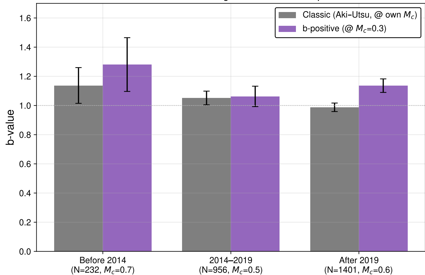
Ulsan Fault b-value through time: classic vs b-positive
