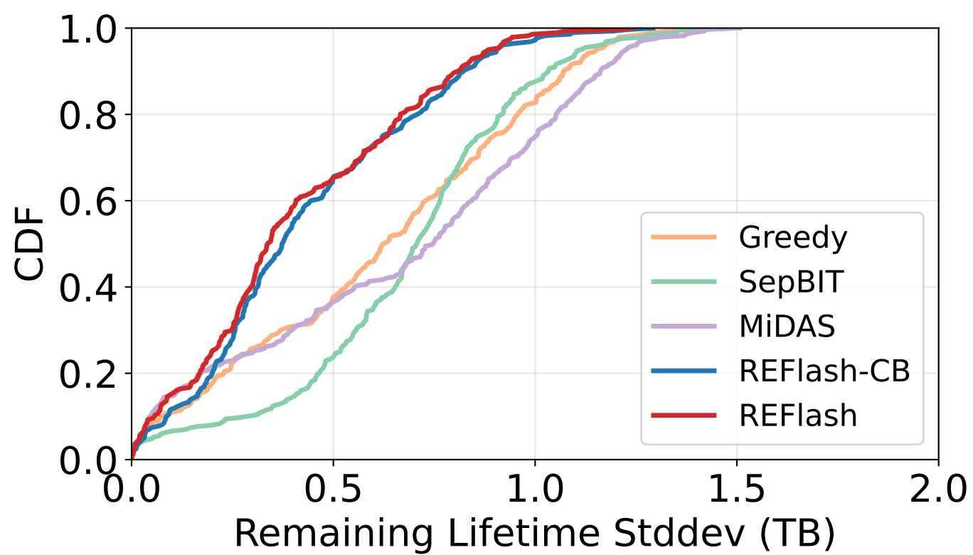
(a) Remaining lifetime stddev per segment
