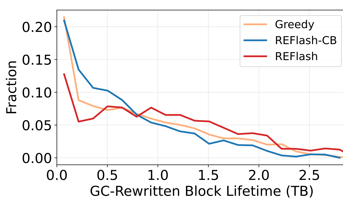
(b) GC-rewritten block lifetime distribution
