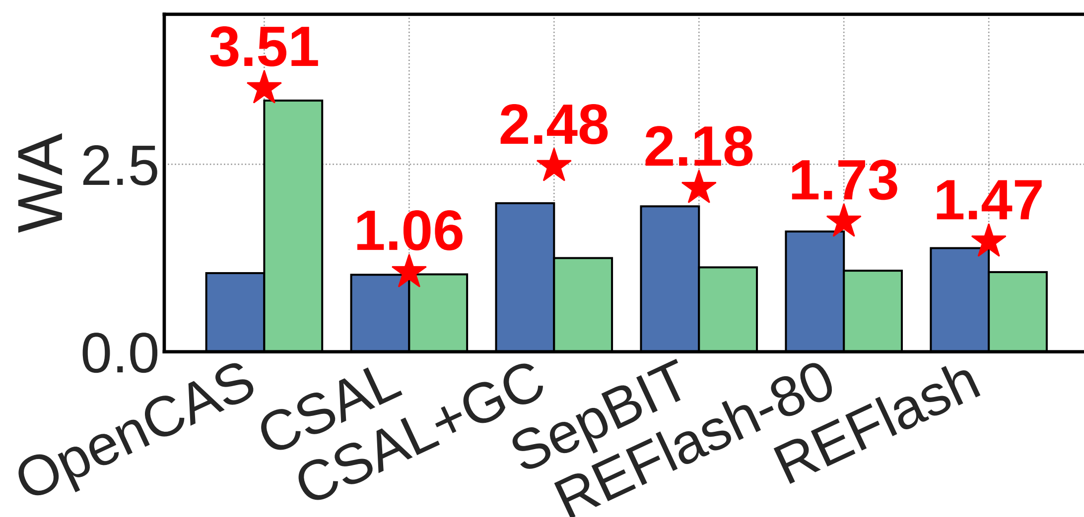
(c) Alibaba1
