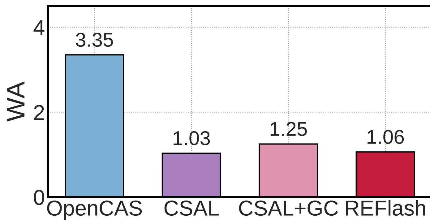
(a) Buffer-tier device WA
