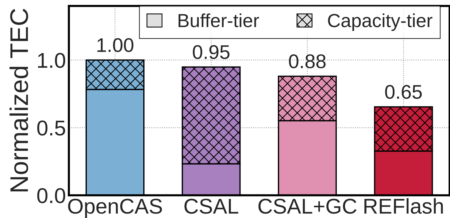
(c) Total endurance cost
