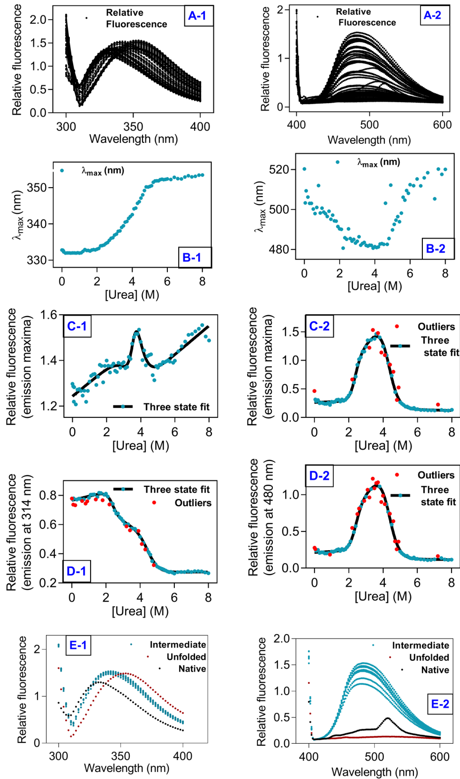
Figure 2. Urea induced unfolding studies of human aldose reductase (hAR) monitored by fluorescence. (A1) Trp fluorescence scans and (A2) ANS fluorescence scans for all the samples. (B1) \lambda_{\max} (Trp fluorescence) and (B2) \lambda_{\max} (ANS fluorescence) against [urea]. (C1) I_{\max} (Trp fluorescence) and (C2) I_{\max} (ANS fluorescence) against [urea]. (D1) I_{295/314} (Trp fluorescence) and (D2) I_{370/480} (ANS fluorescence) against [urea]. (E1) Trp fluorescence and (E2) ANS fluorescence of samples in native (black), intermediate (cyan), and unfolded state (red). Solid lines represent curves fitted to the unfolding transitions; filled symbols represent data points from unfolding experiments; red symbols represent outliers.
