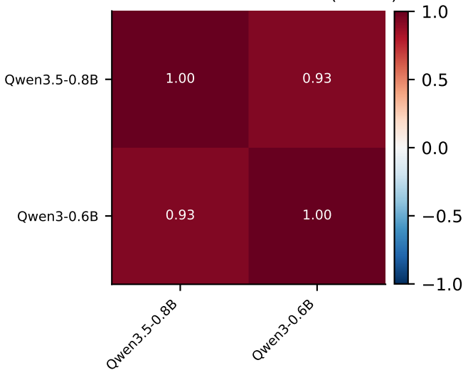
Retrieval-score correlation (sorted)
