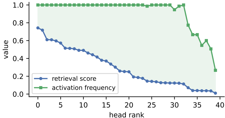
Qwen3.5-0.8B always-active heads: 30
