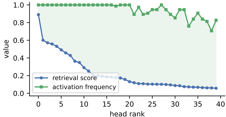
Qwen3-0.6B always-active heads: 21
