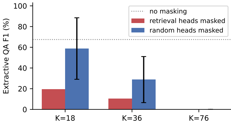
Extractive QA F1 with and without masking
