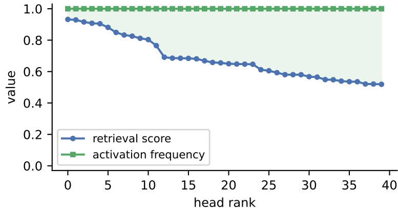
Qwen3-0.6B always-active heads: 92
