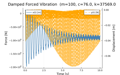
(c) Total
