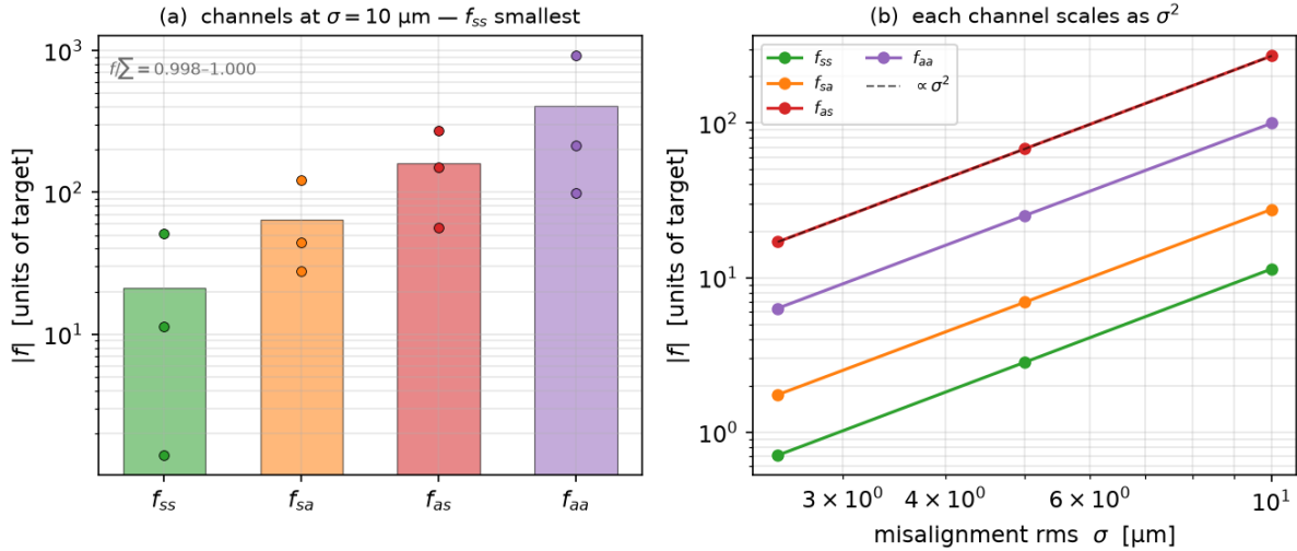
FIG. 2. The four false-EDM channels of Eq. (8), measured by projecting the misalignments and tracking each part separately. (a) At \sigma = 10 \mu\text{m} the pure-symmetric channel f_{ss} is the smallest, and every channel containing an antisymmetric factor is larger (bars: mean of three seeds; dots: individual seeds; the spread reflects the signed, bilinear character of f ). (b) Each channel scales as \sigma^2 . The four signed channels sum to the full signal within 0.1%.
