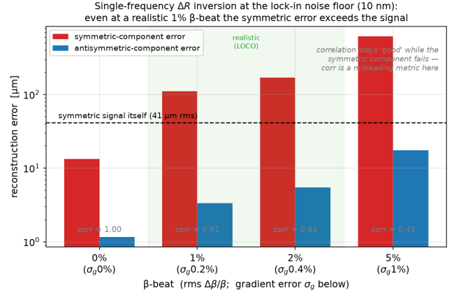
FIG. 4. Difference-orbit inversion at the synchronous-detection noise floor (10 nm, 40 seeds): reconstruction error of the symmetric and antisymmetric components versus the \beta -beat (the driving gradient error \sigma_g is \approx 5\times smaller, shown below each label). The dashed line marks the size of the symmetric signal itself, and the shaded band the realistic LOCO range ( \sim 1 –2% \beta -beat). Already at 1% the symmetric error exceeds the signal, while the Pearson correlation (gray labels) stays misleadingly high; even at zero \beta -beat the conditioning leaves the symmetric error an order of magnitude above the antisymmetric one.
