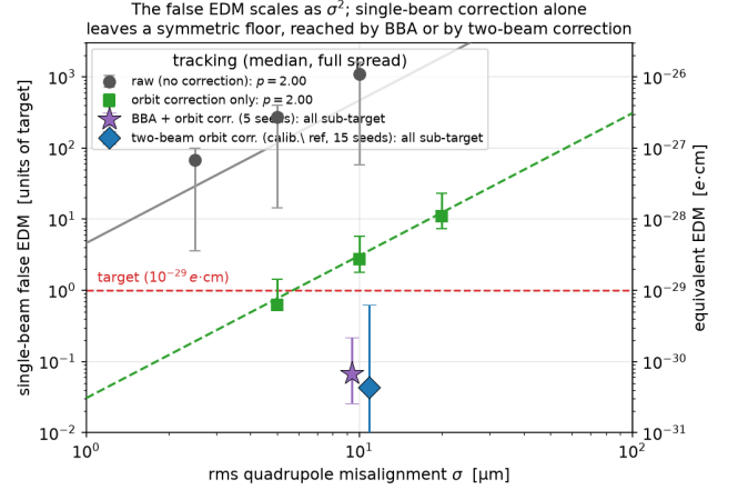
FIG. 3. The single-beam false EDM versus rms misalignment (tracking; median and full spread). Circles: the raw pattern (no correction). Squares: orbit correction alone, which removes the antisymmetric channels but leaves the symmetric floor — still a few times the target at \sigma = 10\ \mu\text{m} . Both scale as \sigma^2 ( p = 2.00 at each stage), confirming the geometric-phase origin; the fit verifies the scaling, not an absolute floor, since at fixed \sigma the false EDM varies by more than an order of magnitude with the symmetric/antisymmetric content of the pattern (Sec. III B). The symmetric floor is reached below target by two independent routes at \sigma = 10\ \mu\text{m} (fixed \text{rcond} = 0.01 ). Star: beam-based alignment followed by one orbit correction (median 0.07\times , worst 0.22\times , five seeds; Table III). Diamond: two-beam counter-rotating orbit correction against a calibrated reference, no BBA, at a realistic 1% \beta -beat (median 0.043\times , worst 0.62\times , fifteen seeds; Table II and Sec. VC). The diamond is the odd remnant \frac{1}{2}|f_{\text{CW}} - f_{\text{CCW}}| ; both routes place the residual well below the target.
