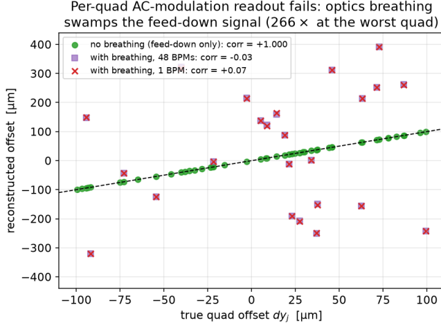
FIG. 5. Per-quadrupole gradient modulation read as an amplitude: reconstructed versus true offsets. The reconstruction is exact when the optics breathing is artificially removed (green), but uncorrelated with it present, whether one BPM (red) or all 48 (purple) are used — the breathing, coherent with the modulation, does not average down.
