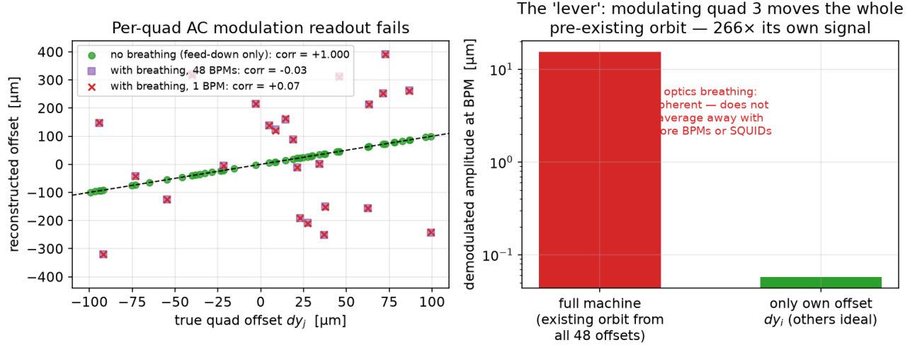
FIG. 5. Per-quadrupole gradient modulation read as an amplitude. Left: reconstructed versus true offsets — exact when the optics breathing is artificially removed (green); uncorrelated with it present, whether one BPM (red) or all 48 (purple) are used. Right: the demodulated amplitude responds to the re-transported pre-existing orbit at 266\times the level of the quadrupole’s own feed-down signal; the contamination is coherent and does not average down.
