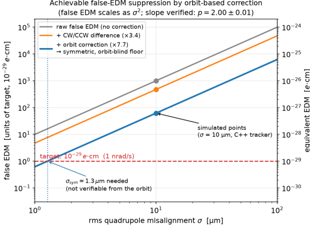
FIG. 4. Main result: the false EDM reachable by orbit correction versus the rms quadrupole misalignment. The points at \sigma = 10 \mu\text{m} are C++ tracking; all curves scale as \sigma^2 ( p = 2.00 ). The corrected floor crosses the target only at \sigma_{\text{sym}} \approx 1.3 \mu\text{m} — a level no orbit measurement can verify.
