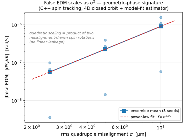
FIG. 2. Validation of the false-EDM estimator: the measured |dS_y/dt| scales as \sigma^{2.00} across \sigma = 2.5\text{--}10 \mu\text{m} (C++ tracking, three seeds per point) — the fingerprint of a pure geometric phase with no linear leakage. The scatter between seeds reflects that f is a product dx \cdot dy : individual patterns can happen to be small.
