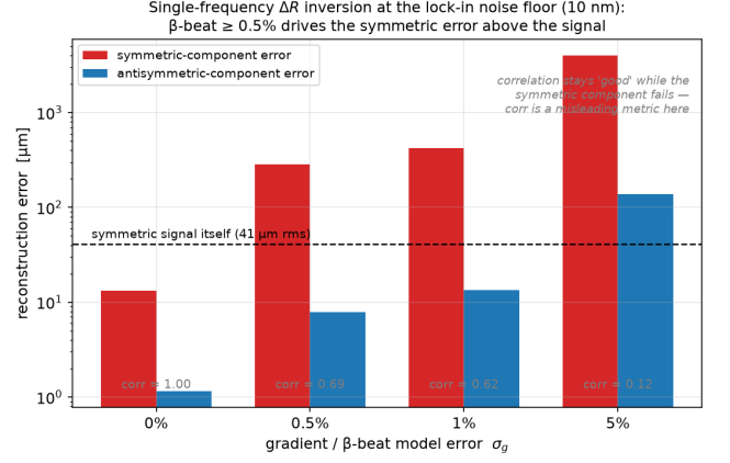
FIG. 5. Single-frequency \Delta R inversion at the lock-in noise floor (10 nm, 40 seeds). Symmetric and antisymmetric reconstruction errors versus the optics-model error \sigma_g ; the dashed line is the symmetric signal itself. Any realistic model error ( \geq 0.5\% ) pushes the symmetric error far above the signal while the correlation (gray labels) stays deceptively high — the correlation trap of Sec. II E.
