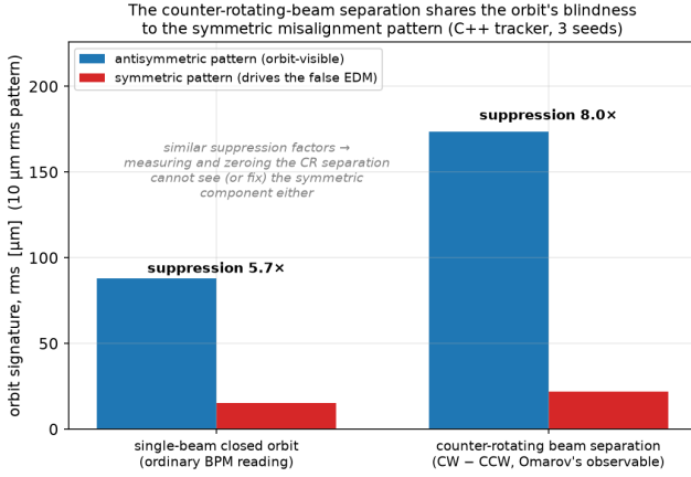
FIG. 6. The counter-rotating beam separation (right group) suppresses the symmetric pattern by a factor similar to the ordinary single-beam orbit (left group): as an orbit observable it shares the orbit's blindness to the component that drives the residual false EDM.
