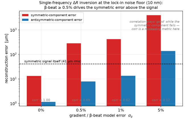
FIG. 4. Difference-orbit inversion at the synchronous-detection noise floor (10 nm, 40 seeds): reconstruction error of the symmetric and antisymmetric components versus the optics-model error. The dashed line marks the size of the symmetric signal itself. A model error at the realistic \geq 0.5\% level drives the symmetric error far above the signal while the Pearson correlation (gray labels) remains high.
