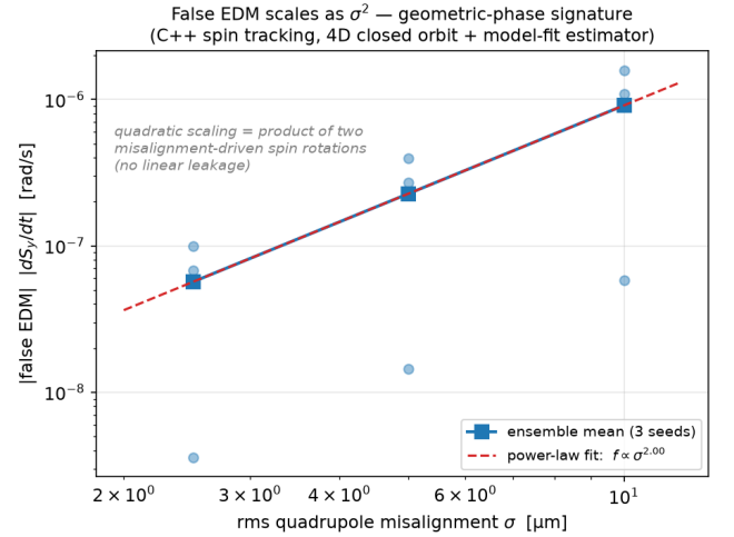
FIG. 2. Validation of the false-EDM estimator: the measured |dS_y/dt| scales as \sigma^{2.00} across \sigma = 2.5 –10 \mu\text{m} (C++ tracking, three seeds per point) — the fingerprint of a pure geometric phase with no linear leakage. The scatter between seeds reflects that f is a product dx \cdot dy : individual patterns can happen to be small.
