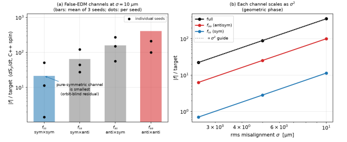
FIG. 1. The four false-EDM channels of Eq. (10), measured with the C++ spin tracker. (a) At \sigma = 10 \mu\text{m} the pure-symmetric channel f_{ss} is the smallest; every channel containing the antisymmetric part is larger (bars: mean of three seeds; dots: individual seeds — the per-seed scatter reflects the bilinear, signed nature of f ). (b) Each channel scales as \sigma^2 , the signature of the geometric phase. Orbit correction removes the antisymmetric part, collapsing all channels but f_{ss} .
