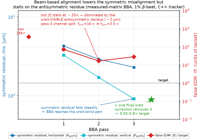
FIG. 7. Beam-based alignment lowers the symmetric misalignment but stalls on the antisymmetric residue (measured-matrix BBA under 1% \beta -beating, C++ tracking). Blue/cyan (left axis): the symmetric residual of the two planes falls steadily with each pass, the vertical one below the target-equivalent level — BBA reaches the orbit-blind component that response-matrix inversion cannot. Red (right axis): the false EDM |f| nonetheless stalls near 20\times the target, because it is dominated by the orbit-visible antisymmetric residue ( \sim 2\ \mu\text{m} ), the centering error remaining at BBA’s precision floor (largest in the horizontal plane) once the measured-matrix steering of Sec. VB has done its work; the channel decomposition of the third-pass residual gives f_{\text{anti}} = 16\times \gg f_{\text{sym}} = 3.5\times . A single final orbit correction removes that residue (green star), bringing |f| below the target for this seed.
