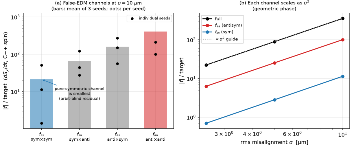
FIG. 3. The four false-EDM channels of Eq. (8), measured by projecting the misalignments and tracking each part separately. (a) At \sigma = 10 \mu m the pure-symmetric channel f_{ss} is the smallest, and every channel containing an antisymmetric factor is larger (bars: mean of three seeds; dots: individual seeds; the spread reflects the signed, bilinear character of f ). (b) Each channel scales as \sigma^2 . The four signed channels sum to the full signal within 0.1%.
