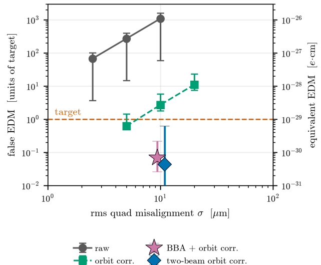
FIG. 3. The single-beam false EDM versus rms misalignment (tracking; median and full spread). Circles: the raw pattern (no correction). Squares: orbit correction alone, which removes the antisymmetric channels but leaves the symmetric floor — still a few times the target at \sigma = 10\text{ }\mu\text{m} . Both scale as \sigma^2 ( p = 2.00 at each stage), confirming the geometric-phase origin; the fit verifies the scaling, not an absolute floor, since at fixed \sigma the false EDM varies by more than an order of magnitude with the symmetric/antisymmetric content of the pattern (Sec. III B). The symmetric floor is reached below target by two independent routes at \sigma = 10\text{ }\mu\text{m} (fixed \text{rcond} = 0.01 ). Star: beam-based alignment followed by one orbit correction (median 0.07\times , worst 0.22\times , five seeds; Table II). Diamond: two-beam counter-rotating orbit correction against a calibrated reference, no BBA, at a realistic 1% \beta -beat (median 0.043\times , worst 0.62\times , fifteen seeds; Table I and Sec. V C). The diamond is the odd remnant \frac{1}{2}|f_{\text{CW}} - f_{\text{CCW}}| ; both routes place the residual well below the target.
