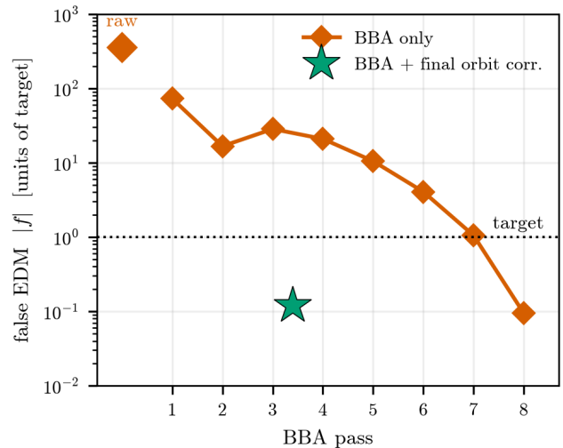
FIG. 6. Beam-based alignment drives the false EDM below target without a plateau (measured-matrix BBA under a conservative 1% rms gradient error, \approx 5\% \beta -beat, eight passes, C++ tracking). Diamonds: the false EDM |f| from the raw machine ( 356\times target) through eight BBA passes; it falls monotonically past the third pass and crosses below target by the eighth ( 0.09\times ). It does not plateau; the descent is merely slow, because BBA grinds the symmetric residual down magnet by magnet, reaching the orbit-blind component that a single-beam response-matrix inversion cannot. A final orbit correction removes the orbit-visible antisymmetric residue collectively, reaching the target in about three passes instead of eight (green star: five-seed ensemble, median 0.07\times , all sub-target).
