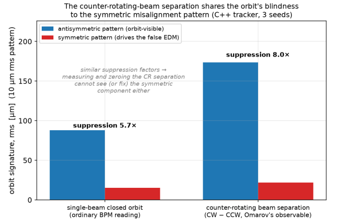
FIG. 6. The counter-rotating beam separation (right group) suppresses the symmetric pattern by a factor similar to the ordinary single-beam orbit (left group): as an orbit observable it shares the orbit's blindness to the component that drives the residual false EDM.
