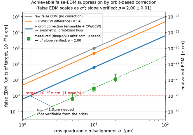
FIG. 1. False EDM before and after orbit-based correction versus the rms quadrupole misalignment. The three lines (raw, +CW/CCW, +orbit correction) are anchored at the ensemble median of tracking results at \sigma = 10\ \mu\text{m} (several random misalignment patterns per stage, not a single seed). The green squares are directly measured orbit-corrected residuals (deep truncated-SVD correction, median and full spread of three random seeds at each of \sigma = 5, 10, 20\ \mu\text{m} ); the dashed line is their power-law fit, |f| \propto \sigma^p with p = 2.00 , confirming the quadratic scaling empirically over a factor of four in \sigma . (These measured points use a deeper correction on favorable seeds than the ensemble line, so they verify the slope rather than the absolute floor.) Each line should be read as the center of a band rather than a curve: at fixed \sigma the false EDM varies by more than an order of magnitude with the symmetric/antisymmetric content of the pattern (Sec. III C), so the rms alone does not determine the signal.
