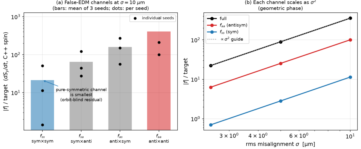
FIG. 3. The four false-EDM channels of Eq. (8), measured by projecting the misalignments and tracking each part separately. (a) At \sigma = 10 \mu\text{m} the pure-symmetric channel f_{ss} is the smallest, and every channel containing an antisymmetric factor is larger (bars: mean of three seeds; dots: individual seeds; the spread reflects the signed, bilinear character of f ). (b) Each channel scales as \sigma^2 . The four signed channels sum to the full signal within 0.1%.
