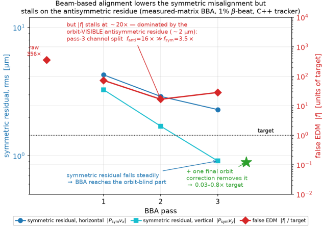
FIG. 7. Beam-based alignment lowers the symmetric misalignment but stalls on the antisymmetric residue (measured-matrix BBA under 1% \beta -beating, C++ tracker). Blue/cyan (left axis): the symmetric residual of the two planes falls steadily with each pass, the vertical one below the target-equivalent level — BBA reaches the orbit-blind component that response-matrix inversion cannot. Red (right axis): the false EDM |f| nonetheless stalls near 20\times the target, because it is dominated by the orbit-visible antisymmetric residue ( \sim 2\text{ }\mu\text{m} ), the residual centering error at BBA’s precision floor (largest horizontally) — not the analytic-steering failure, which the measured steering matrix has already removed; the channel decomposition of the third-pass residual gives f_{\text{anti}} = 16\times \gg f_{\text{sym}} = 3.5\times . A single final orbit correction removes that residue (green star), bringing |f| below the target for this seed.
