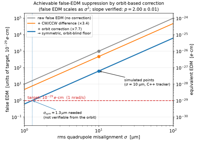
FIG. 3. Main result: the false EDM reachable by orbit-based correction as a function of the rms quadrupole misalignment. Points at \sigma = 10 \mu\text{m} are C++ tracking results; all curves scale as \sigma^2 (verified exponent p = 2.00 ). The corrected floor crosses the target only at \sigma_{\text{sym}} \approx 1.3 \mu\text{m} — a level that no orbit-based measurement can verify.
