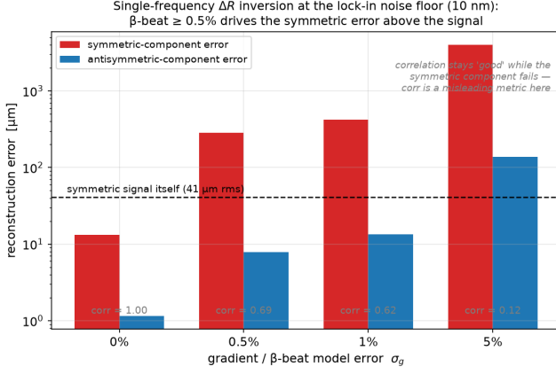
FIG. 4. Single-frequency \Delta R inversion at the lock-in noise floor (10 nm, 40 seeds). Symmetric- and antisymmetric-component reconstruction errors vs. the optics-model error \sigma_g ; the dashed line is the symmetric signal itself. Any realistic model error ( \geq 0.5\% ) drives the symmetric error far above the signal while the Pearson correlation (gray labels) remains deceptively high — the correlation trap of Sec. IID.
