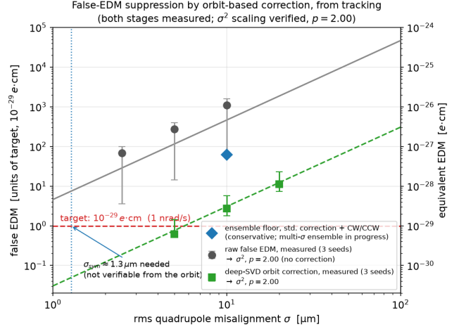
FIG. 1. False EDM before and after orbit-based correction versus the rms quadrupole misalignment, from tracking. Both stages are directly measured points, not drawn curves. Grey circles: the raw false EDM (no correction, median and full spread of three random seeds at \sigma = 2.5, 5, 10\ \mu\text{m} ). Green squares: the residual after a deep truncated-SVD orbit correction (three seeds at \sigma = 5, 10, 20\ \mu\text{m} ). The lines through each are power-law fits |f| \propto \sigma^p with p = 2.00 , confirming the quadratic scaling empirically over a factor of four in \sigma at both stages. The blue diamond marks the conservative ensemble floor of a standard-depth correction with the counter-rotating-beam difference at \sigma = 10\ \mu\text{m} (Table II); the deep-SVD points reach lower, so they bound the slope while the conservative floor bounds the absolute level, and a multi- \sigma ensemble at the standard depth is in progress. The large vertical spread of the measured points is physical: at fixed \sigma the false EDM varies by more than an order of magnitude with the symmetric/antisymmetric content of the pattern (Sec. III C), so the rms alone does not determine the signal.
