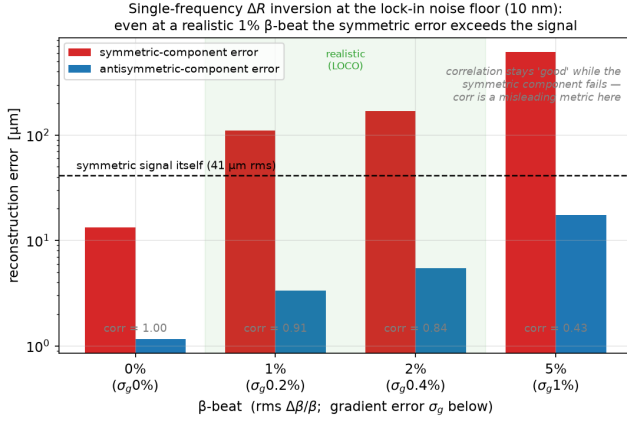
FIG. 5. Difference-orbit inversion at the synchronous-detection noise floor (10 nm, 40 seeds): reconstruction error of the symmetric and antisymmetric components versus the \beta -beat (the driving gradient error \sigma_g is \approx 5\times smaller, shown below each label). The dashed line marks the size of the symmetric signal itself, and the shaded band the realistic LOCO range ( \sim 1 – 2\% \beta -beat). Already at 1% the symmetric error exceeds the signal, while the Pearson correlation (gray labels) stays misleadingly high; even at zero \beta -beat the conditioning leaves the symmetric error an order of magnitude above the antisymmetric one.
