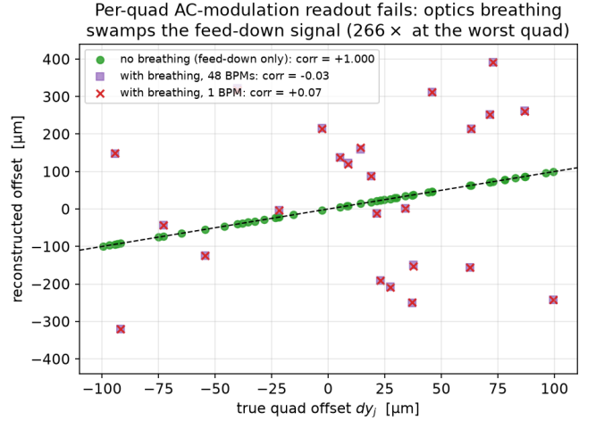
FIG. 6. Per-quadrupole gradient modulation read as an amplitude: reconstructed versus true offsets. The reconstruction is exact when the optics breathing is artificially removed (green), but uncorrelated with it present, whether one BPM (red) or all 48 (purple) are used — the breathing, coherent with the modulation, does not average down.
