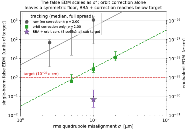
FIG. 4. The single-beam false EDM versus rms misalignment (tracking; median and full spread). Circles: the raw pattern (no correction). Squares: orbit correction alone, which removes the antisymmetric channels but leaves the symmetric floor — still a few times the target at \sigma = 10 \mu\text{m} . Both scale as \sigma^2 ( p = 2.00 at each stage), confirming the geometric-phase origin; the fit verifies the scaling, not an absolute floor, since at fixed \sigma the false EDM varies by more than an order of magnitude with the symmetric/antisymmetric content of the pattern (Sec. III B). Star: the full scheme — beam-based alignment followed by one orbit correction (fixed truncated-SVD depth, \text{rcond} = 0.01 ) — evaluated over five misalignment seeds at \sigma = 10 \mu\text{m} ; all five fall below the target, with median 0.07\times and worst case 0.22\times (Table II).
