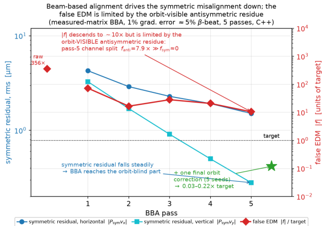
FIG. 3. Beam-based alignment drives the symmetric misalignment down; the false EDM is limited by the antisymmetric residue (measured-matrix BBA under a 1% rms gradient error, \approx 5\% \beta -beat, five passes, C++ tracking). Blue/cyan (left axis): the symmetric residual of the two planes falls steadily with each pass, the vertical one below the target-equivalent level — BBA reaches the orbit-blind component that a single-beam response-matrix inversion cannot. Red (right axis): the false EDM |f| descends to \sim 10\times the target by the fifth pass but is limited there, because at the common few-micron floor it is dominated by the orbit-visible antisymmetric residue; the channel decomposition of the fifth-pass residual gives f_{\text{anti}} \approx 7.9\times against a negligible f_{\text{sym}} . A single final orbit correction removes that residue (green star: five-seed ensemble, median 0.07\times , all sub-target).
