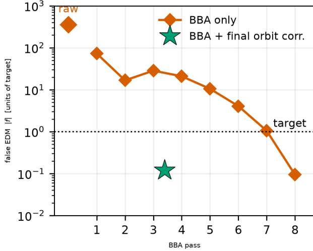
FIG. 6. Beam-based alignment drives the false EDM below target without a plateau (measured-matrix BBA under a conservative 1% rms gradient error, \approx 5\% \beta -beat, eight passes, C++ tracking). Diamonds: the false EDM |f| from the raw machine ( 356\times target) through eight BBA passes; it falls monotonically past the third pass and crosses below target by the eighth ( 0.09\times ). It does not plateau; the descent is merely slow, because BBA grinds the symmetric residual down magnet by magnet, reaching the orbit-blind component that a single-beam response-matrix inversion cannot. A final orbit correction removes the orbit-visible antisymmetric residue collectively, reaching the target in about three passes instead of eight (green star: five-seed ensemble, median 0.07\times , all sub-target).
