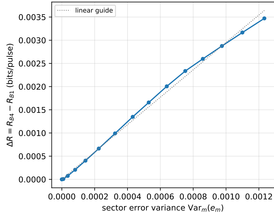
(c) Gain tracks the Jensen-gap source term
