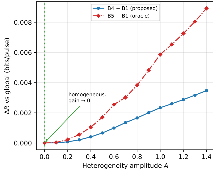
(b) Gain appears only with heterogeneity
