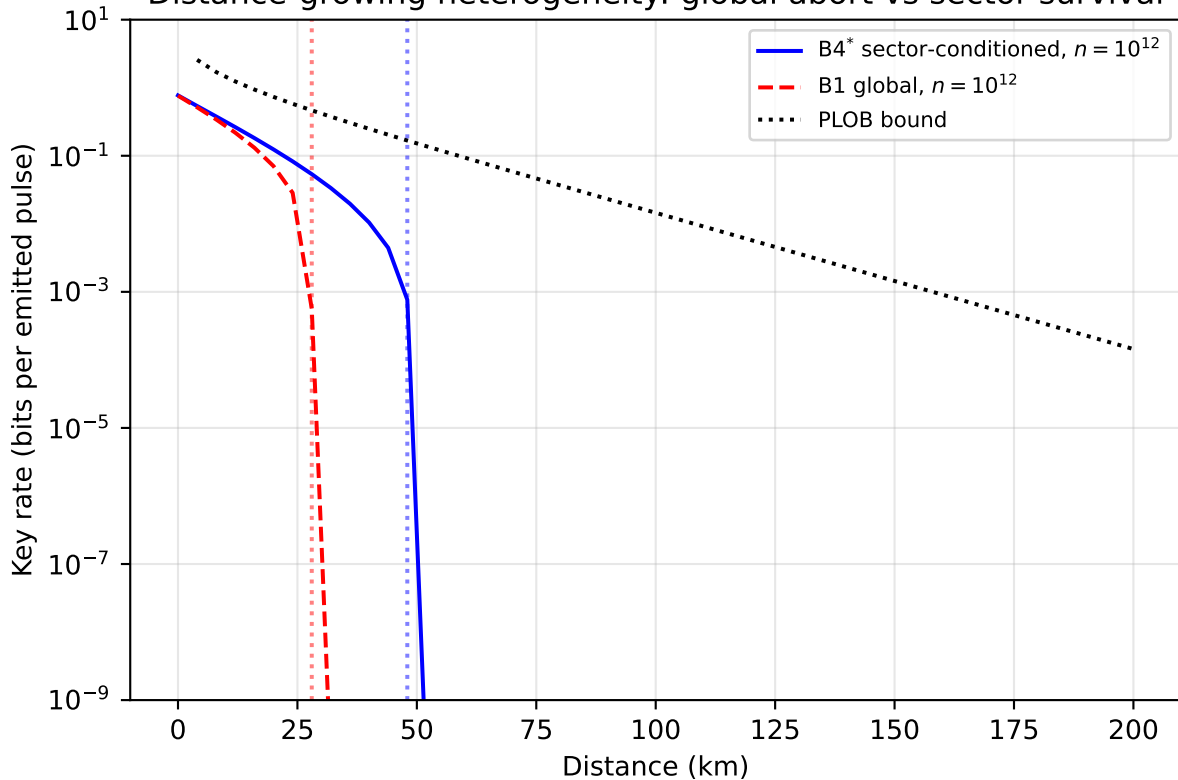
Distance-growing heterogeneity: global abort vs sector survival
