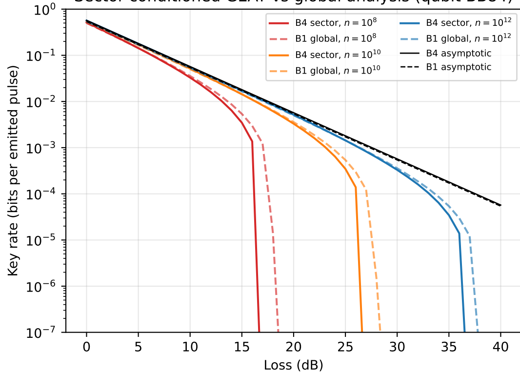
Sector-conditioned GEAT vs global analysis (qubit BB84)
