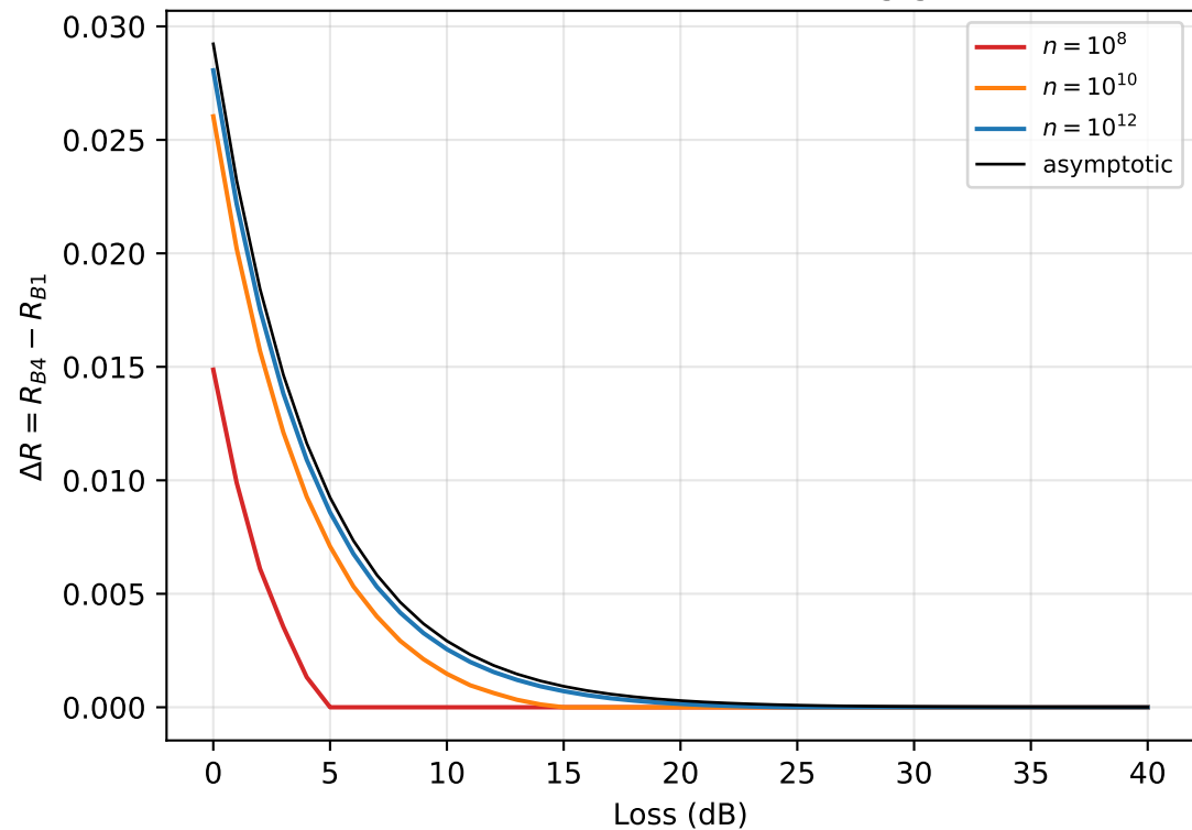
Finite-size sector-conditioning gain
