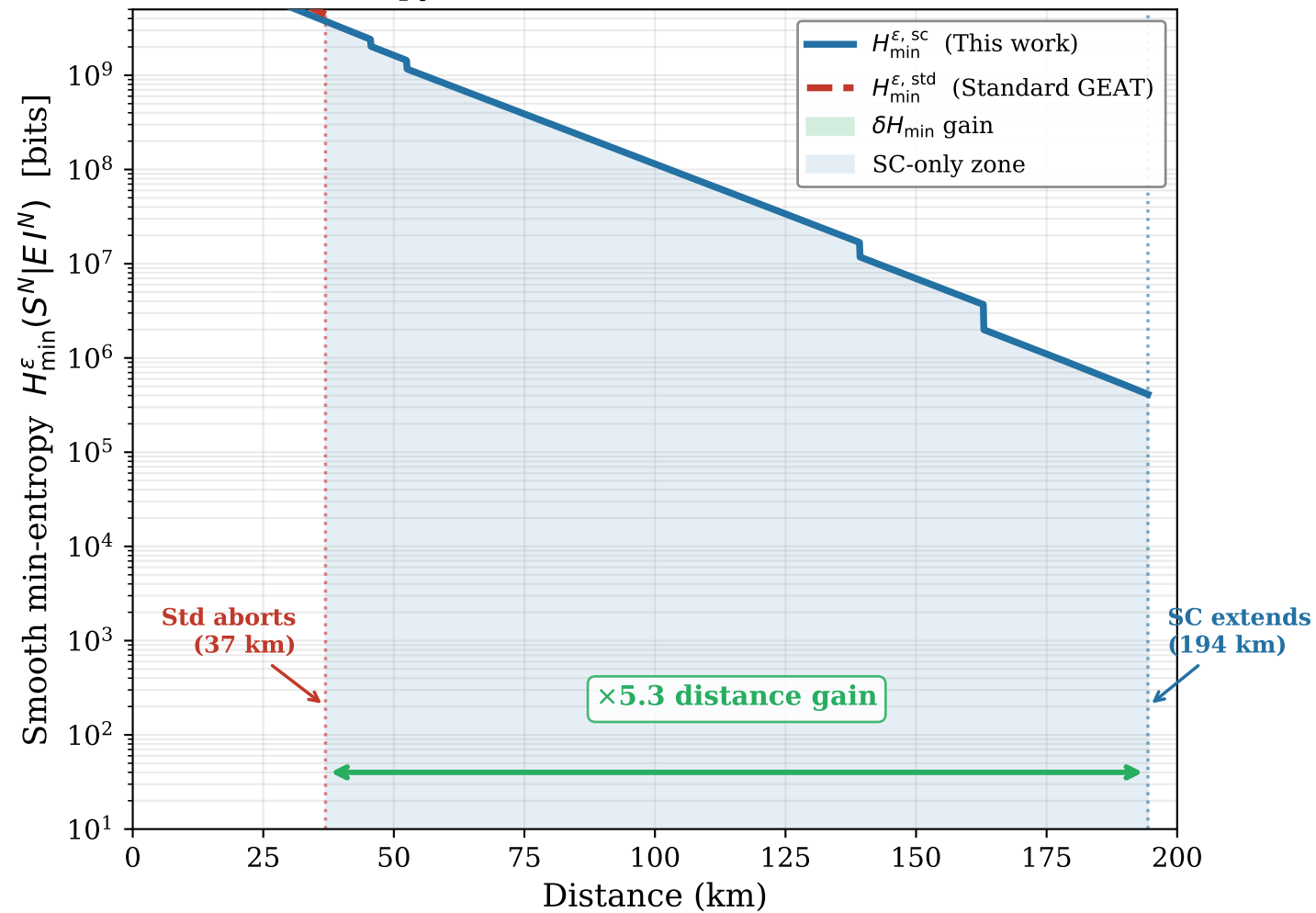
(a) Min-entropy: sector-conditioned vs. standard ( N=10^{12} )
