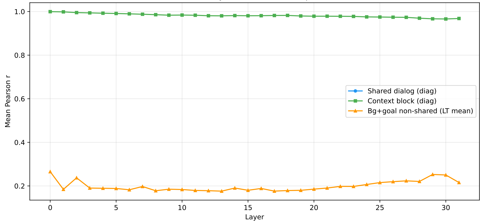
RSA across layers — Turn 0→1 — Episode 26
