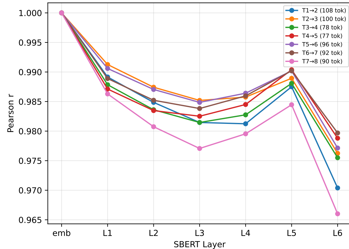
Diagonal mean
