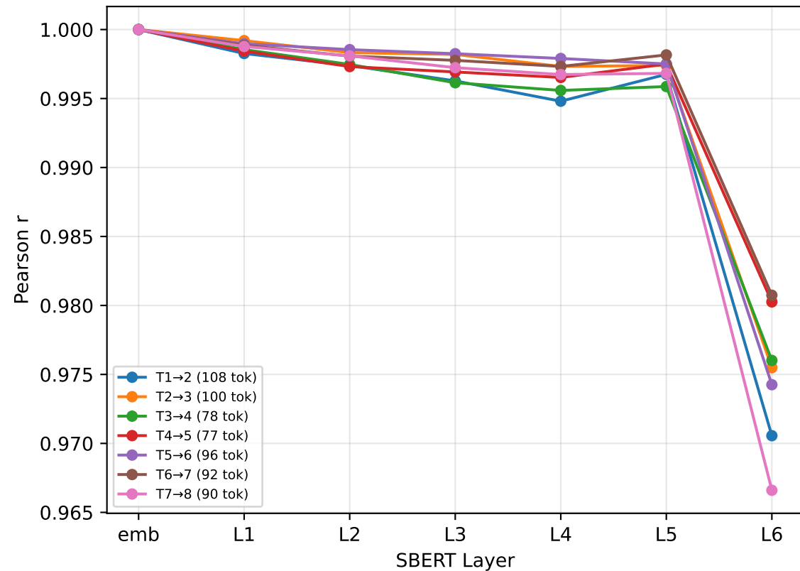
Mean-pool
