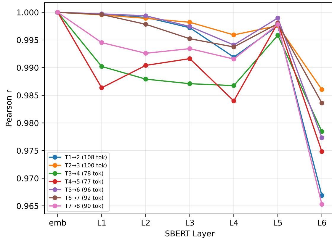
Last-token
