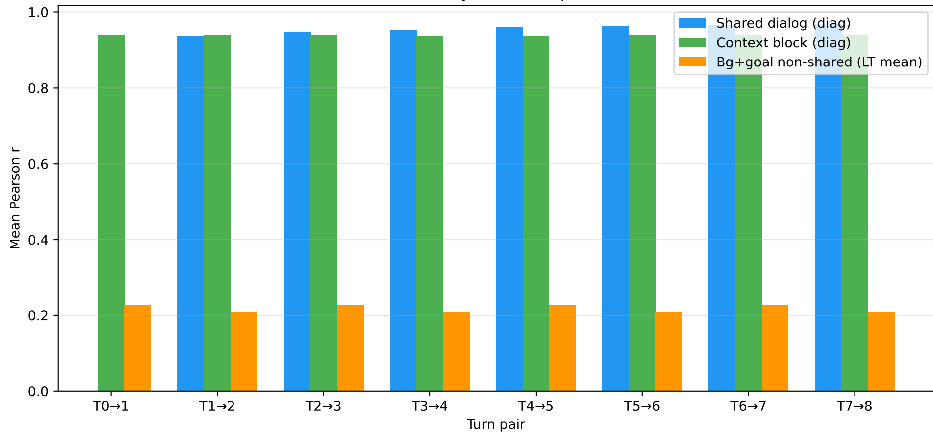
RSA at last layer (31) — Episode 46
